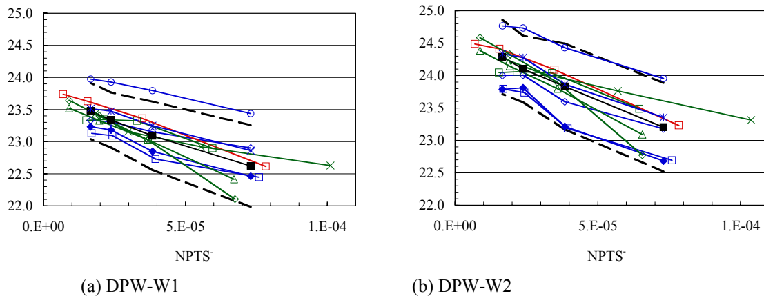
Figure 11: Comparison of lift-to-drag ratio for DPW-W1 and DPW-W2.
