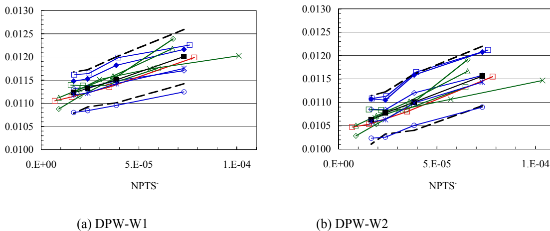
Figure 12: Comparison of idealized profile drag coefficient for DPW-W1 and DPW-W2.
