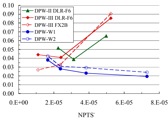
(a) Pressure Drag Coefficient
