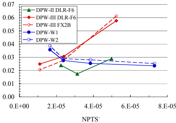
(a) Total Drag Coefficient
